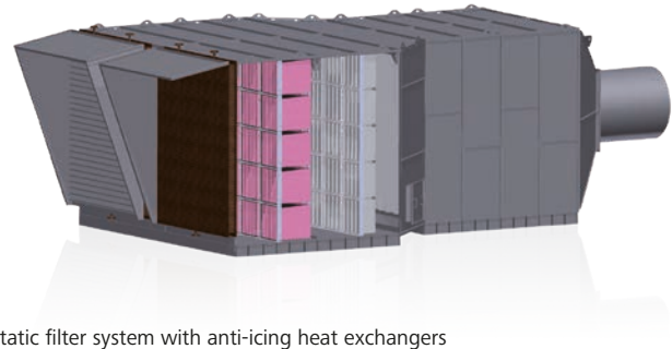
Static filter system with anti-icing heat exchangers
