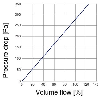
Pressure drop diagram
